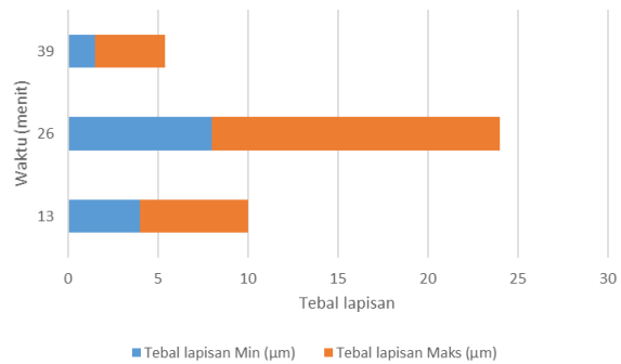
Gambar 4. Ketebalan hasil proses electroplating
