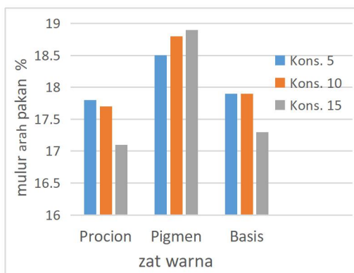
Gambar 8. Histogram mulur kain arah pakan
