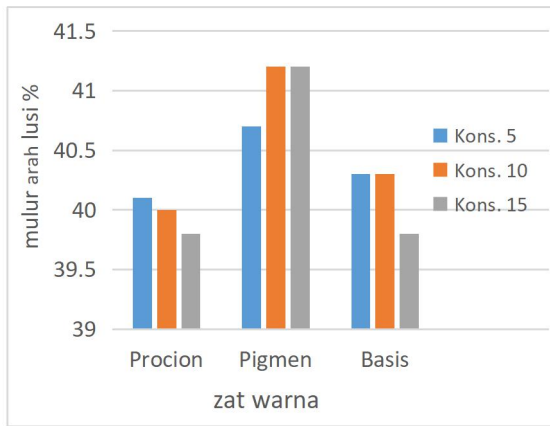
Gambar 7. Histogram mulur kain arah lusi
